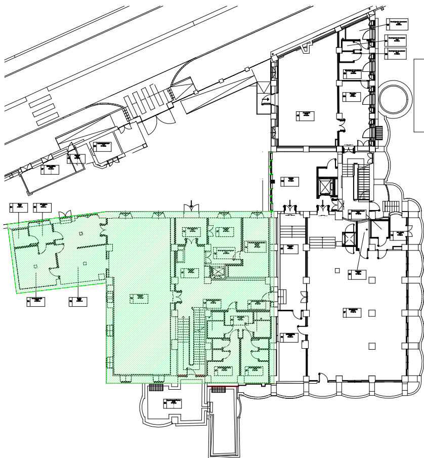
Piano seminterrato
